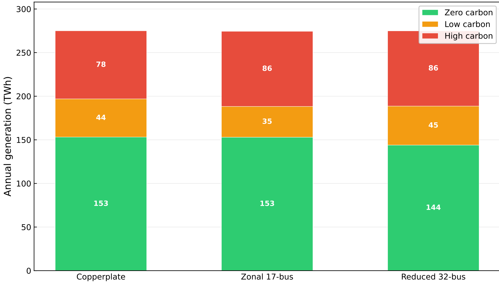
Annual Generation by Energy Group — GB 2023
